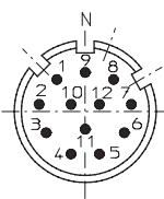
12 pin plug
