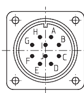
10 pin plug
