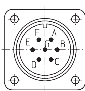
7 pin plug
